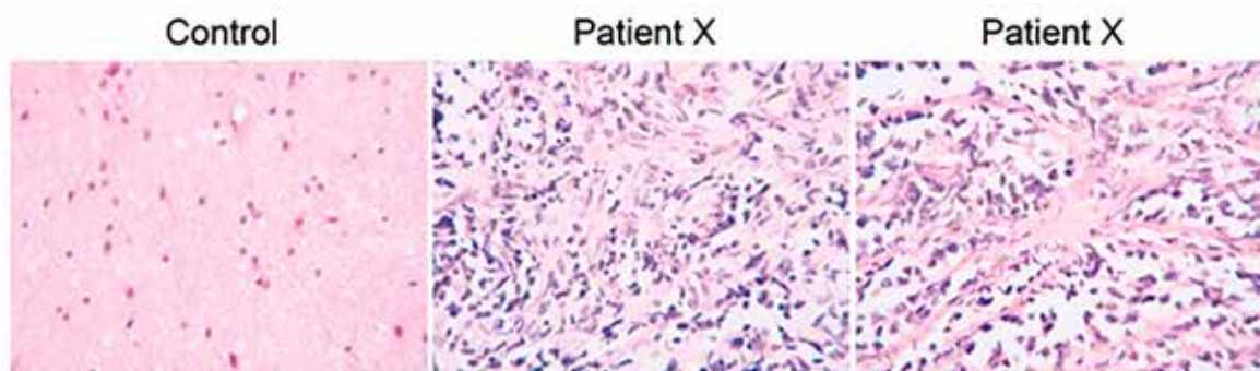
Fig. 1. The morphology of the studied tissues. The tissue sections were stained with hematoxylin and eosin, as described elsewhere. Tissue sample of the Patient X is diagnosed as medulloblastoma. Magnification is x400.
